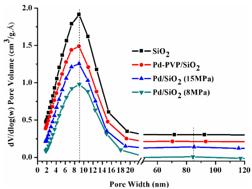
Fig. S2. Pore size distribution curves.
