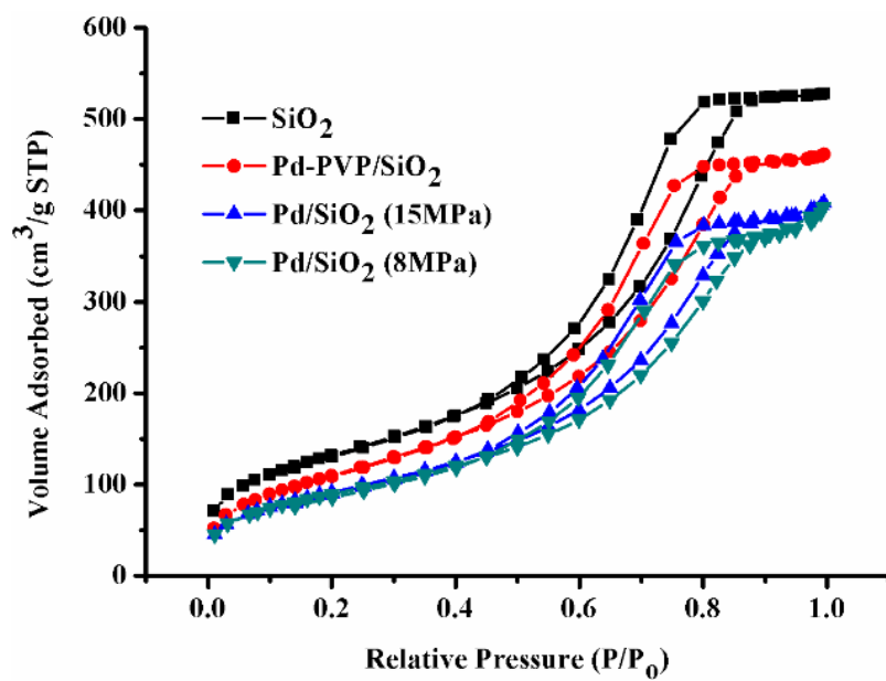
Fig. S1. N 2 adsorption and desorption isotherms
