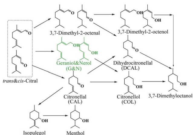
Scheme 1 Reaction pathway of hydrogenation of citral.
