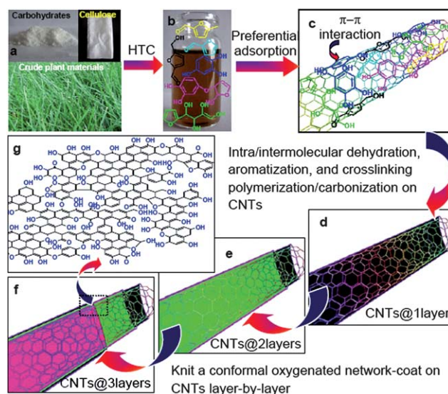
Fig. 1 (a,b) Hydrothermal treatment of a series of biomass gives rise to a mixture solution of heterocyclic/cyclic aromatic compounds (a small typical part of chemicals was listed on bottle); (c–f) the schematic behaviours and knitting mechanism of the aromatic compounds on surface of the CNTs; (g) the schematic structure and compositions of the knitted layer.
