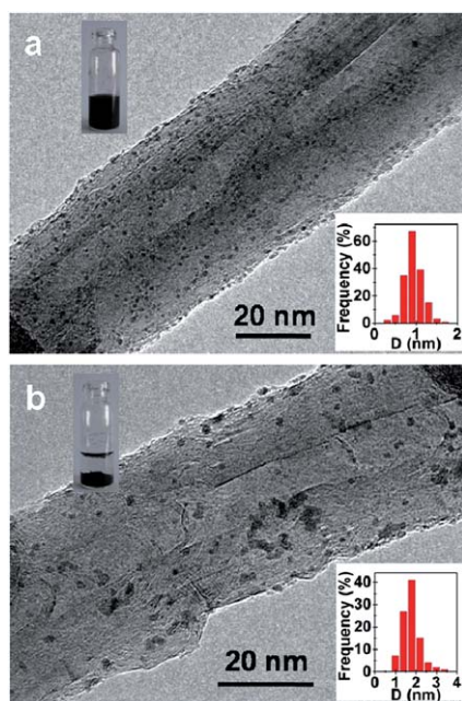
Fig. 4 TEM images of 1.5 wt% Ru/f-CNTs (a) and 1.2 wt% Ru/p-CNTs (b), the size distribution of Ru nanoparticles and the dispersion ability of catalyst in water (inset).
