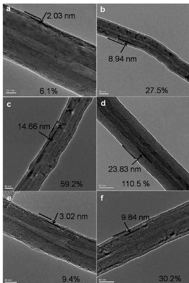
Fig. 2 HRTEM images of f-CNTs functionalized at 180 °C (a–d) for 4 h, 6 h, 8 h, 11 h with the use of glucose; (e,f) with the use of grass and cellulose, respectively. Inset is the thickness and percentage loading of the knitted layer. The percentage loading = (m_{f-CNTs} - m_{p-CNTs})/m_{p-CNTs} ; m_{f-CNTs} = the weight of f-CNTs, m_{p-CNTs} = the weight of CNTs before functionalization.
