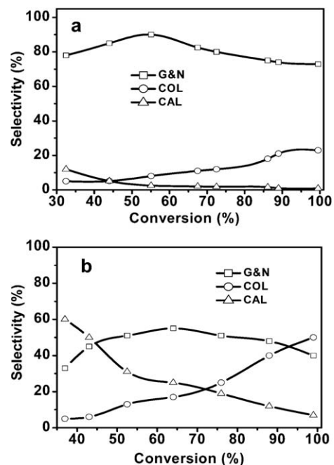
Fig. 5 Plots of selectivity vs. conversion for the selective hydrogenation of citral over 1.5 wt% Ru/f-CNTs (a) and 1.2 wt% Ru/p-CNTs (b).
