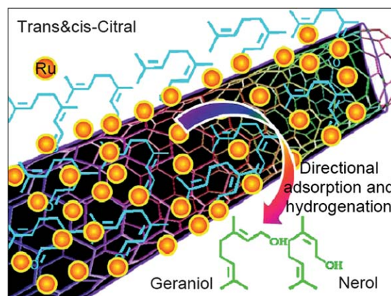
Fig. 6 The probable directional adsorption and hydrogenation of trans - & cis -citral on 1.5 wt% Ru/f-CNTs catalyst in water.
