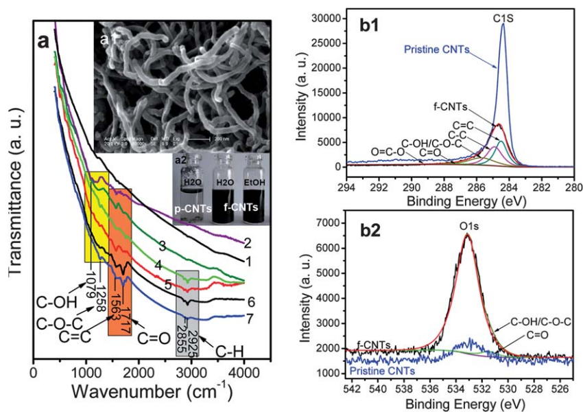
Fig. 3 (a) FTIR spectra of p-CNTs (1) and f-CNTs with different thickness of layers (2–7: 2.03, 3.02, 8.94, 9.84, 14.66, 23.83 nm, respectively) or functionalized with different precursors (2,3,6,7: glucose; 4: grass; 5: cellulose). Inset is the FESEM images of f-CNTs (6), and the picture of dispersion ability of p-CNTs and f-CNTs in solvent. (b1, b2) Comparing the XPS (C1s, O1s) of p-CNTs and f-CNTs (6).
